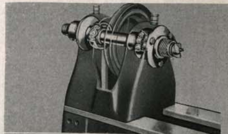
Photo D—Phantom shows how bearings are mounted in head stock. The SKF Ball Bearing at the front end, where the greatest load comes, is the double-row preloaded type. A single type is used at the other end. Note large diameter of shaft.
