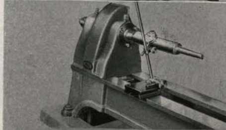
Photo E—Frequent tests are made during manufacture to assure utmost precision. Here a delicate gauge is used to check accuracy of the spindle. This will be recognized as a severe test, the reading being taken at a distance from the spindle. In this position any error is magnified. Following this test the tail stock (with center removed) is slid up to this test bar to check alignment of the tail stock with the head stock.
