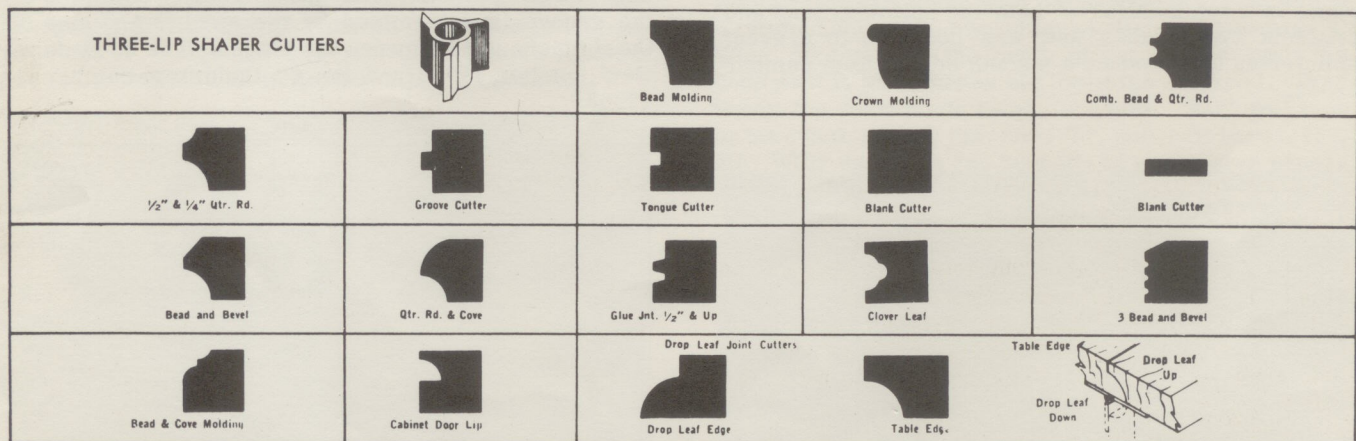
PROFILES OF 3-LIP SHAPER CUTTERS
