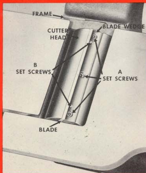
Above photo shows the complete blade coverage and guard coverage, also the accessibility of operating mechanism. Compact, sturdy, precise, precision built.
