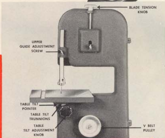
Photo shows the accessibility of the table tilting trunnions, locking mechanism and totally enclosed unit of special all-cast aluminum alloy.
