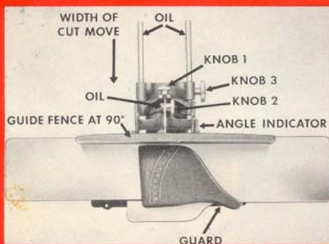
Photo indicates the ease of adjusting SHOPMASTER Blades, which insures more accuracy.
