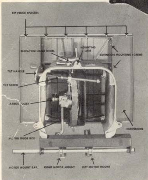
Base view of this saw shows tilting arbor mechanism and motor mount. This picture shows open construction as well as massiveness.
