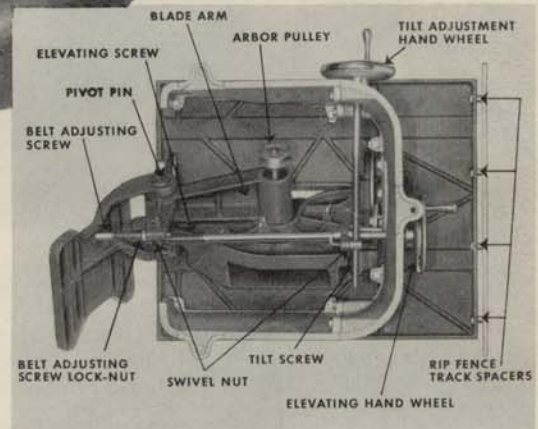
This is view of the tilting arbor mechanism. Motor Mount tilts with arbor. Tilt screws precision machined. Massive construction of arbor casting.
