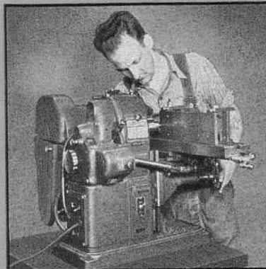
DRILLING — LAYOUT
