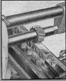
SLABBING
