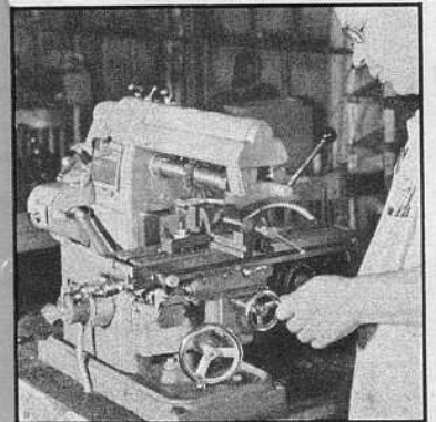
STEP MILLING
