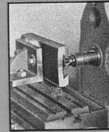
DOVETAILING
