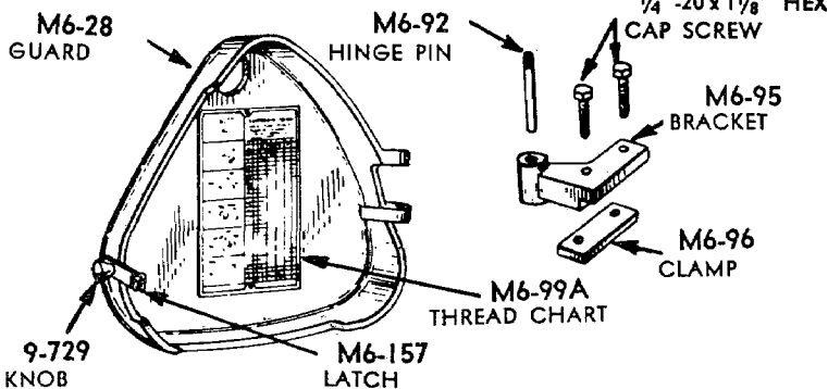
M6-28X GEAR GUARD ASSEMBLY
