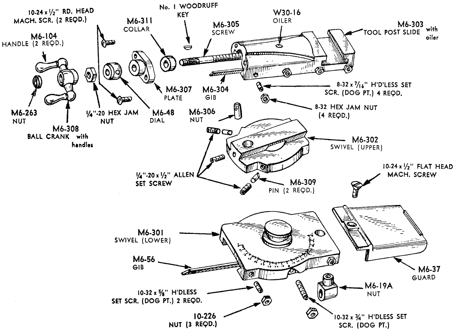
M6-301X COMPOUND REST ASSEMBLY
