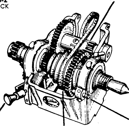
M6-243X BACK GEAR ASSEMBLY Including Spindle Back Gears
