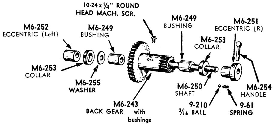
M6-243X BACK GEAR ASSEMBLY Including Spindle Back Gears
