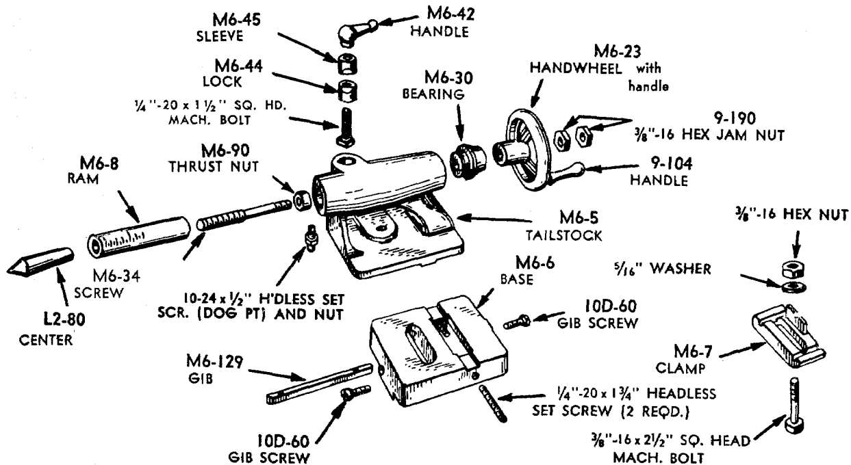
M6-5X TAILSTOCK ASSEMBLY
