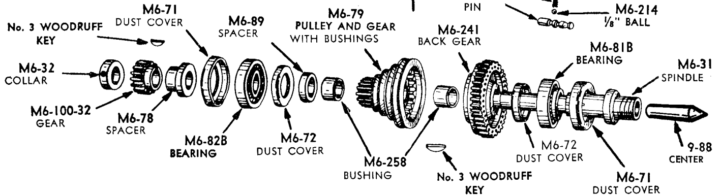
M6-31X SPINDLE ASSEMBLY
