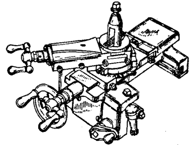
M6-9XY CARRIAGE ASSEMBLY SEE PAGE 4 and 5
