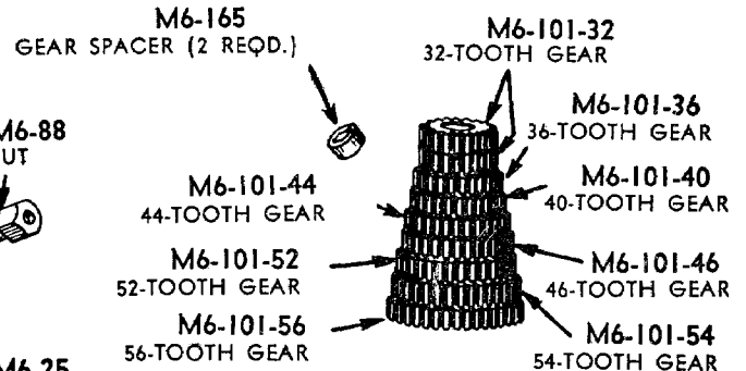
M6-101X CHANGE GEAR ASSEMBLY LESS SPACER
