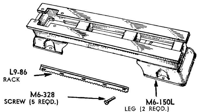
L9-1X BED, LEGS, AND RACK ASSEMBLY
