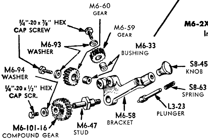
M6-58X TUMBLER ASSEMBLY
