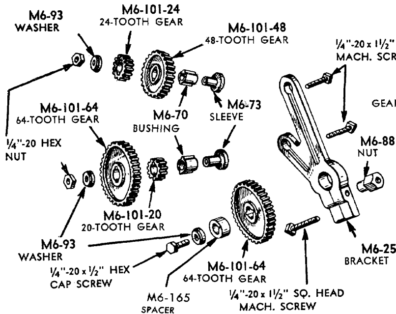
M6-25X CHANGE GEAR BRACKET ASSEMBLY
