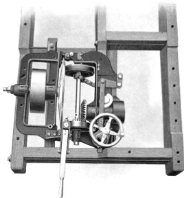
Variable Automatic Disc Friction Feed
