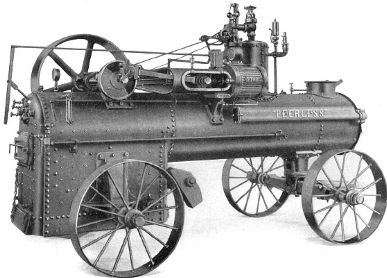
Peerless 50 H. P. Portable Engine
