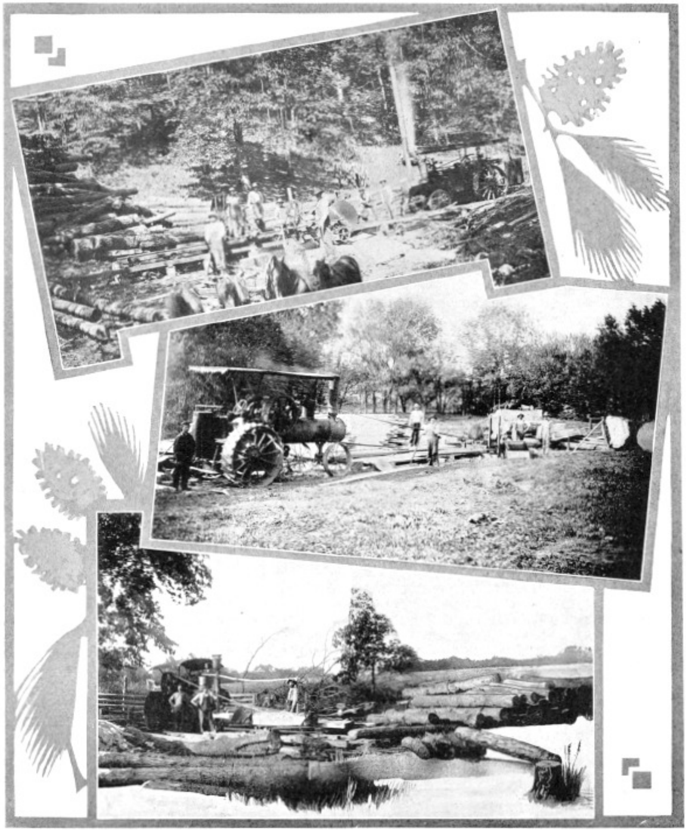
No. 1. Geiser Saw Mill and Peerless Traction Engine in the hills. Geiser Saw Mills.
