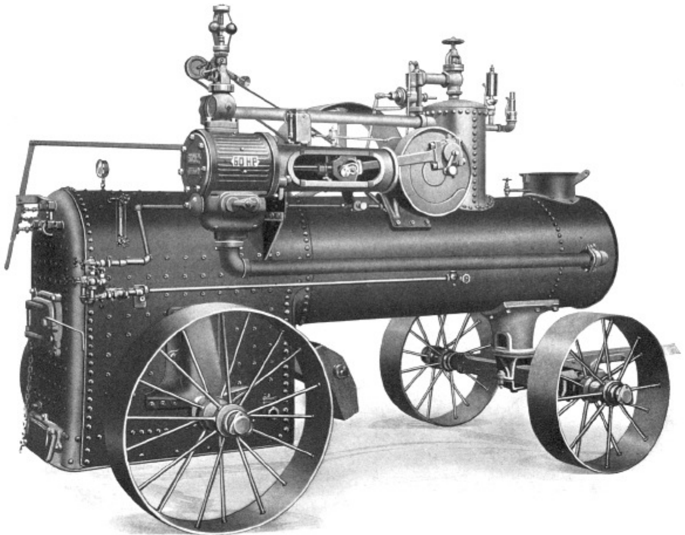
Peerless 60 H. P. Portable Engine
