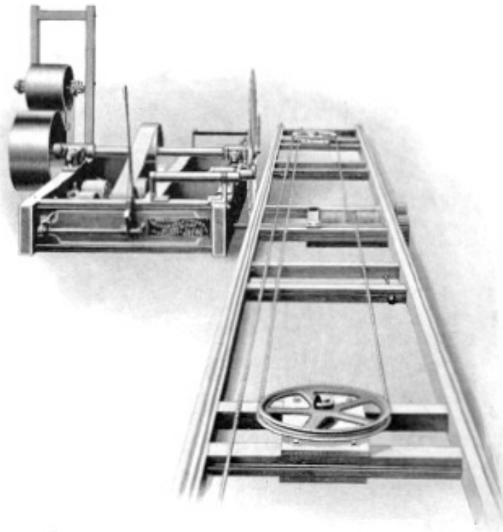
This Cut is Designed to Show How the Cable is Attached to Our Mills, Location of Sheaves, Pulleys, etc.
