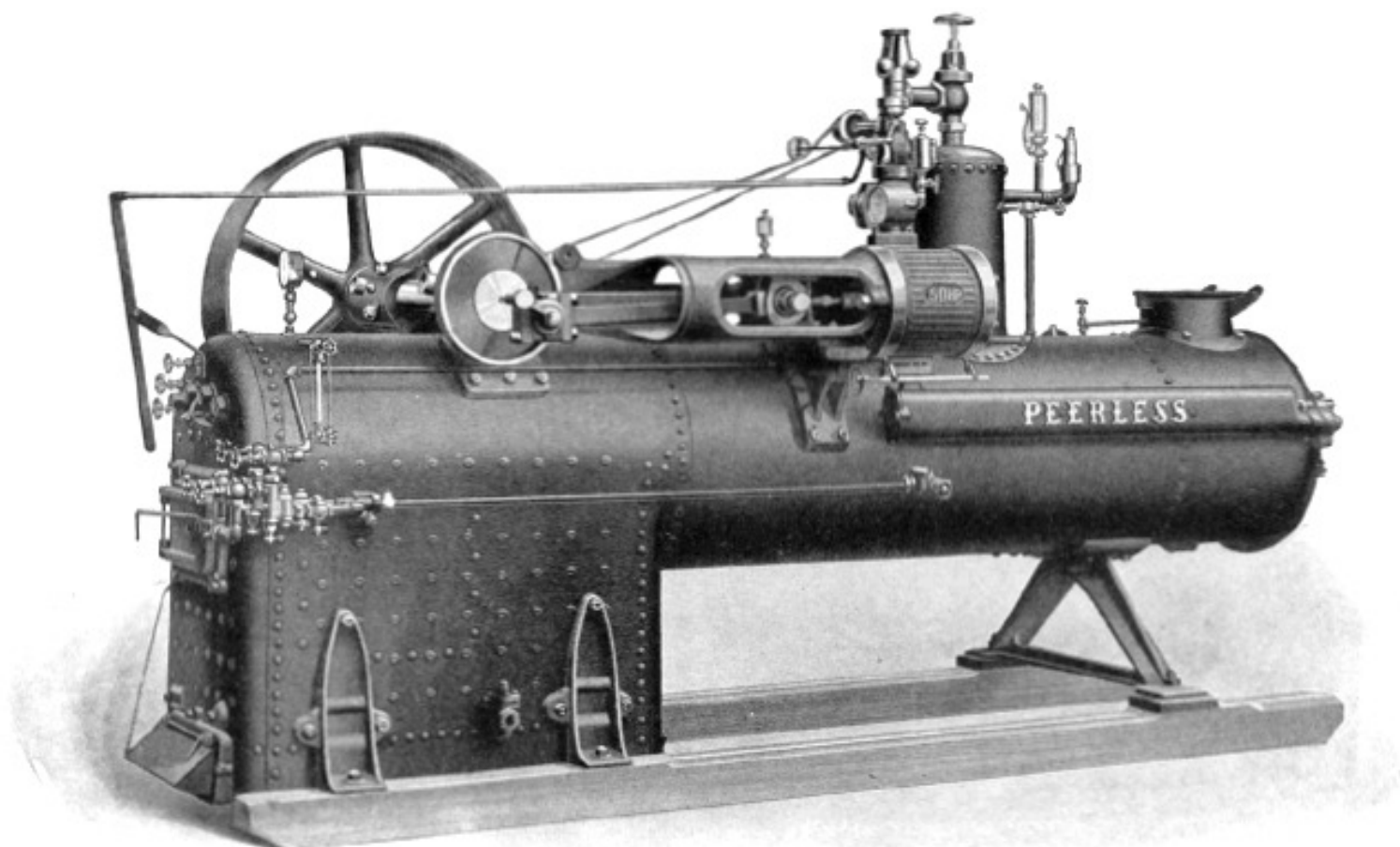
Peerless Portable Engine on Skids Right Side View
