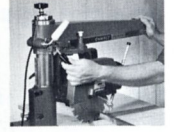
EXCLUSIVE WEDGE-LOK MITER LOCATOR locks positively at 0° and 45°. Scale marked in single degrees.
