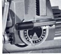
FRONT SINGLE BEVEL CONTROL provides for quick and accurate settings at 0°, 45° and 90°.
