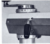
EXCLUSIVE WEDGE-LOK MITER LOCATOR locks positively at 0° and 45°. Scale marked in single degrees.
