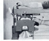
EXCLUSIVE TOP ELEVATION CONTROL gives you precise depth adjustments with eight-section column cap at 1/4" increments.
