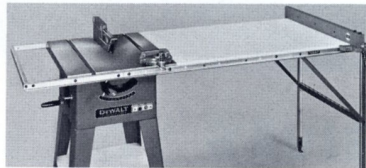
Maximum rip to right: 49" with Extra Wide Extension No. R-137.
