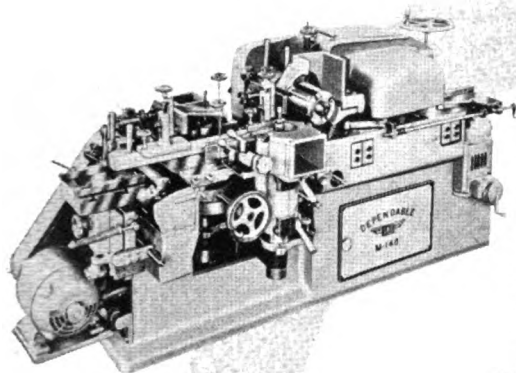
Electro-Unit Drive Moulders; 4" to 10"; speed 20 to 150 ft.; spindle speed up to 6,000. See Dependable Bulletin No. C-12.
