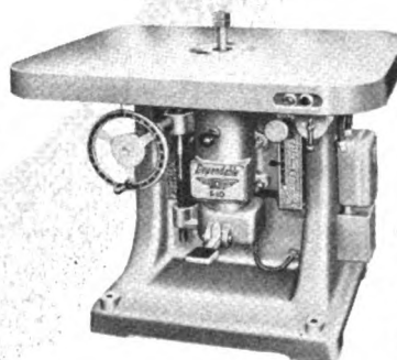
S-10 High Speed Shaper; speeds from 7,000 to 15,000 rpm; write for Dependable Bulletin C-22.
