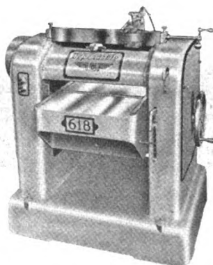
No. 618 and 624 Single Surfacers; modern in design; precision performance unmatched in its price field; ball-bearing throughout. See Bulletin C-32.
