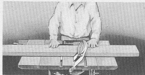
See how easy it is to cut a board at an angle on the CRAFTSMAN Tilting Blade Bench Saw. The table is never tilted, always level and easy to use. The work always lies flat regardless of the angle at which the board is being cut. That means no sliding—much easier operation! A long board which would hit the floor on a tilting table saw is easy to handle on the CRAFTSMAN.
