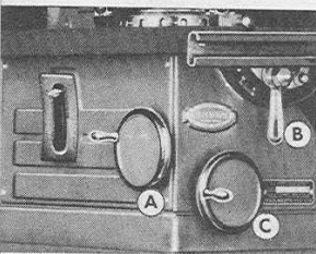
View of controls under table, showing (A) tilting control for adjusting table to any desired angle; (B) positive acting lock on tilting mechanism; (C) control for depth of cut. Controls are at your finger tips.
