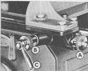
End view of Sears revolutionary new "Roll-over" fence, showing: (A) vernier adjustment; (B) lock on vernier adjustment; (C) main lock for entire fence.
