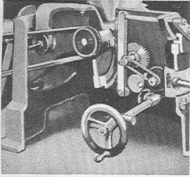
The elevating gears and rack are fully enclosed by two sheet steel sawdust guards. These have been removed in the illustration to show the arrangement of gears which accurately control the tilting mechanism.
