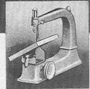
View Showing Table Tilted
