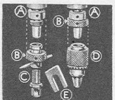
Simplified Tapered Spindles
