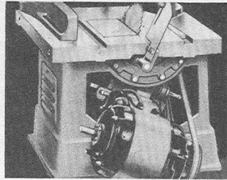
Massive runnions carry the entire tilting blade mechanism. This rugged construction assures real accuracy through many years of hard service. The motor is counterbalanced for ease in operation; it tilts, raises and lowers with saw blade and arbor.
