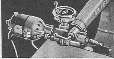
Router head assembly tilted for spindle carving. Scale on head shows angle. Uses cutters below. Does a wide variety of work.
