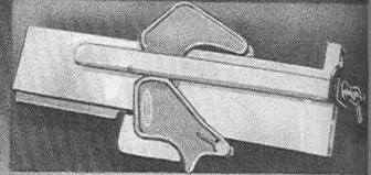
TOP VIEW SHOWING DOUBLE GUARD CONSTRUCTION USED ON THE CRAFTSMAN JOINTER-PLANER
