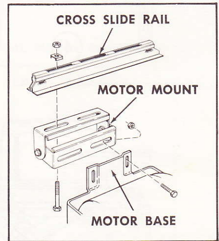
TYPICAL MOTOR MOUNTING
