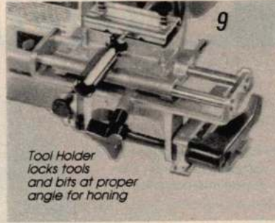
Router Bit Attachment for sharpening high-speed router bits
