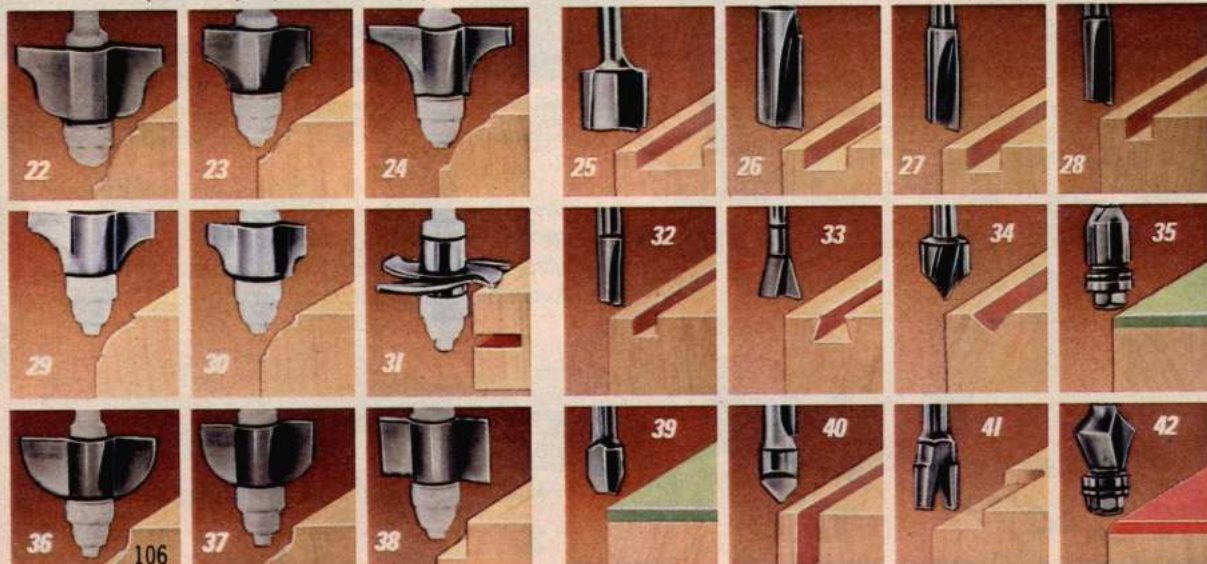
Bits (22 thru 30) require arbor set (43)
