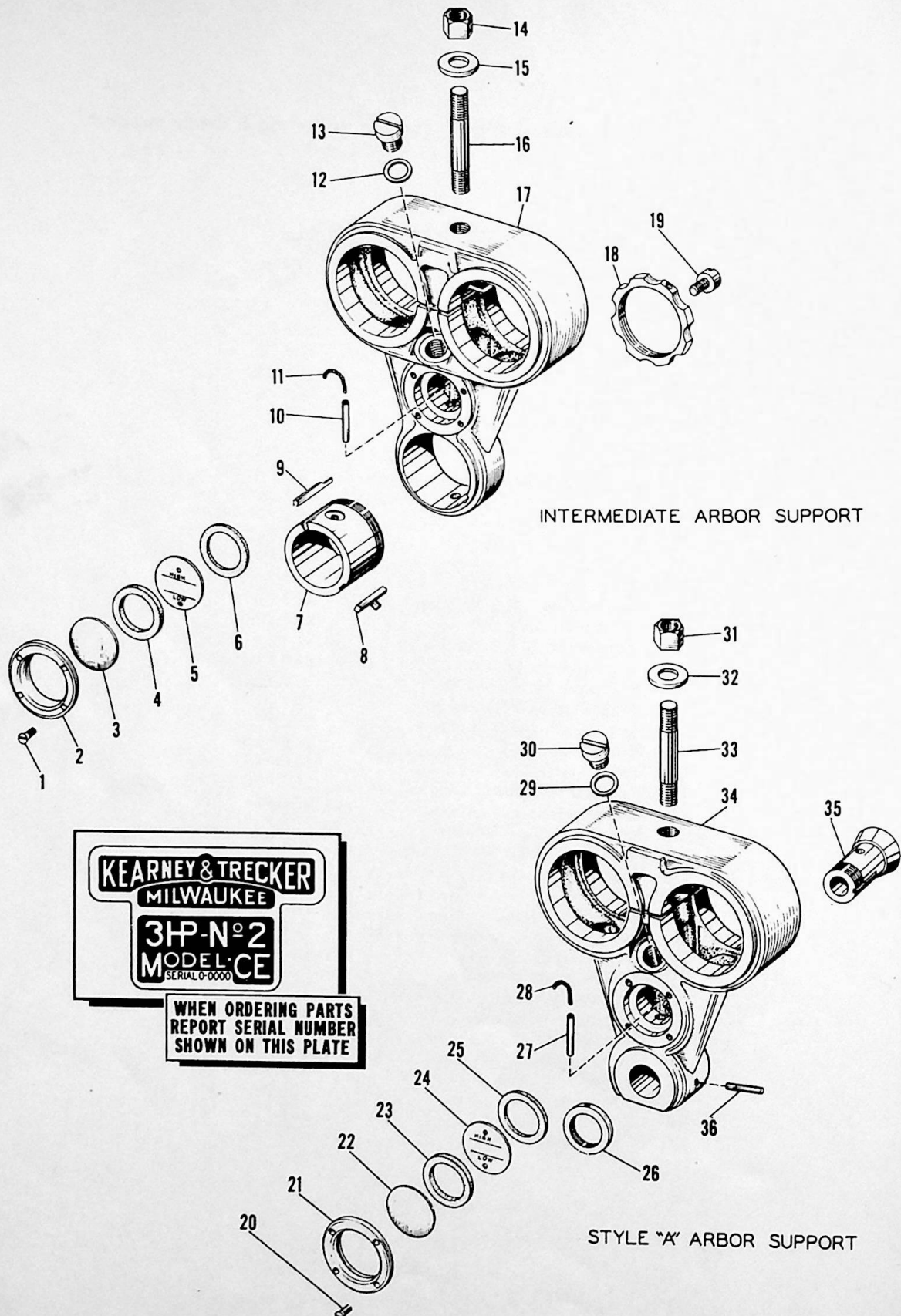
Fig. 17 — Intermediate arbor support and style A arbor support
