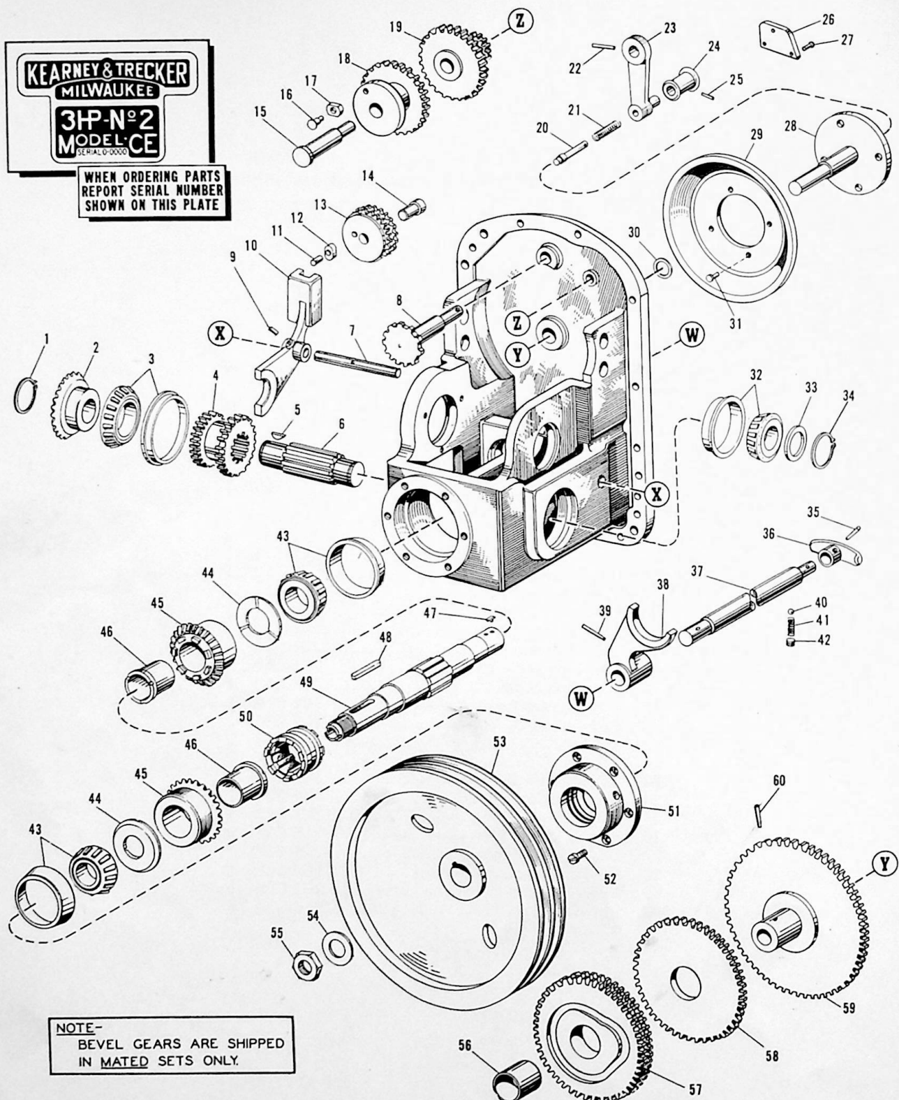
Fig. 6 — Speed gear box assembly — View A
