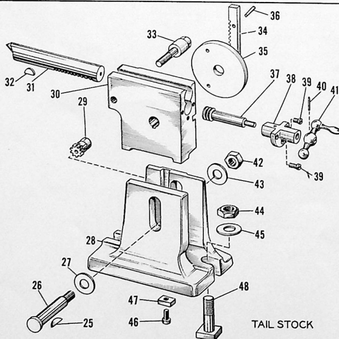
Fig. 18 — Conventional lead attachment, tail stock and steady rest
