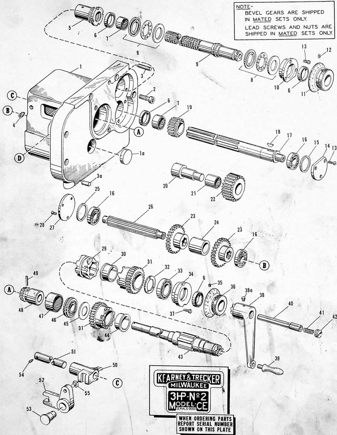
Fig. 9 — Elevating control box assembly
