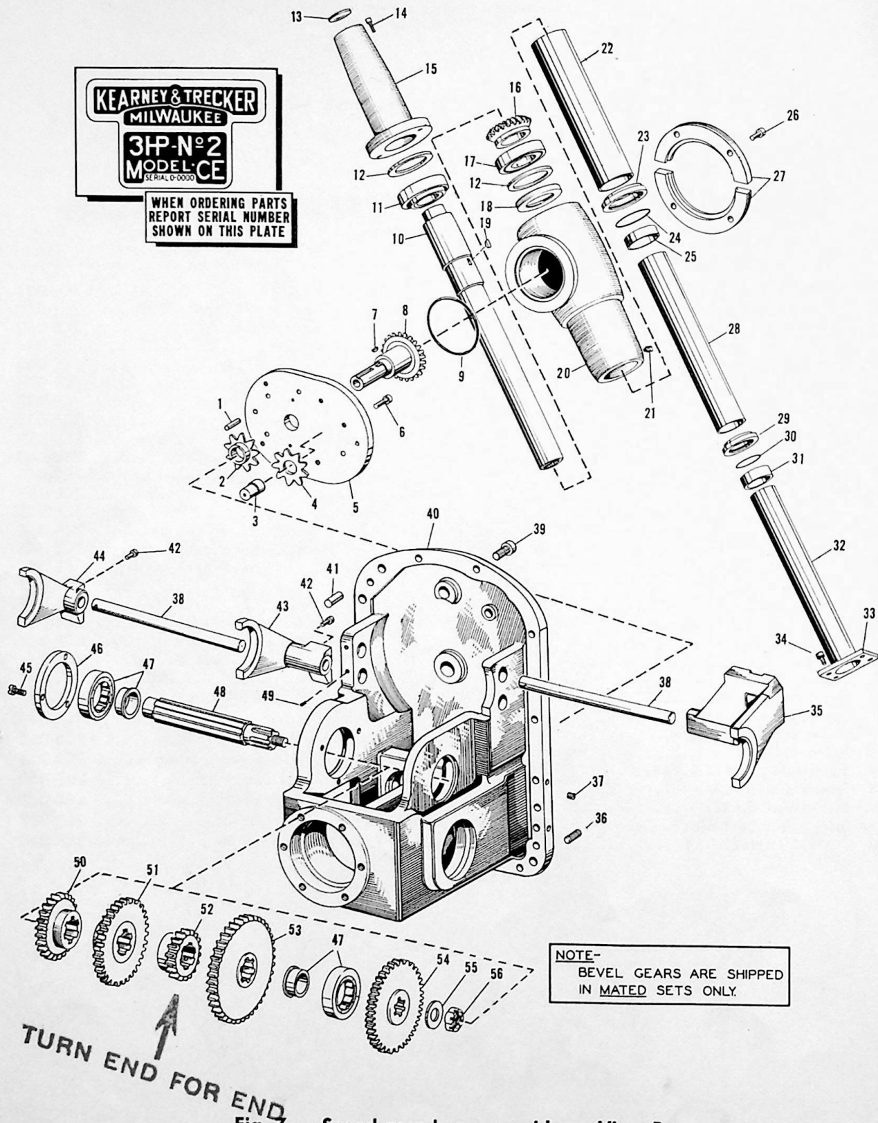
Fig. 7 — Speed gear box assembly — View B
