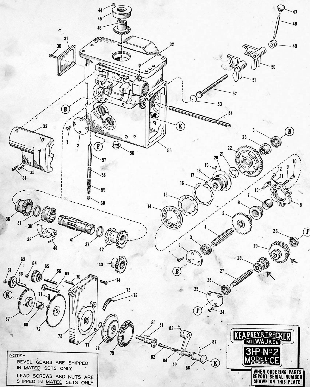
Fig. 10 — Feed gear box assembly — View A
