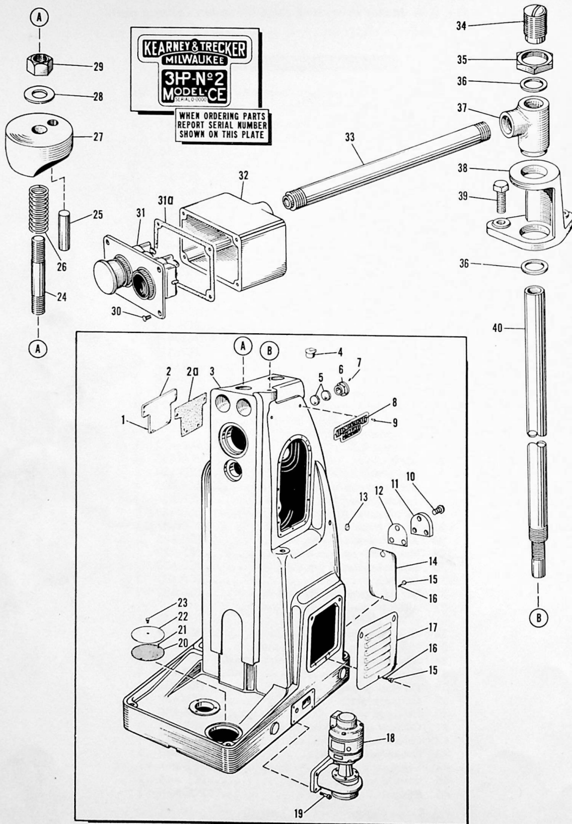
Fig. 4 — Starter assembly and miscellaneous column parts
