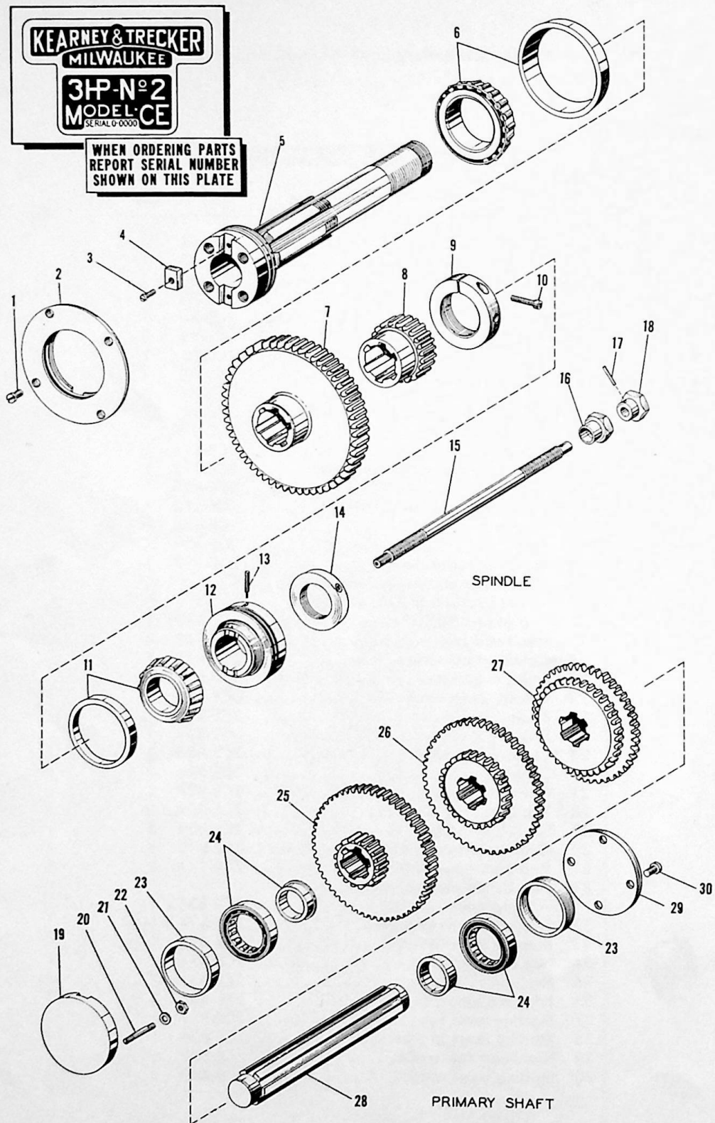
Fig. 5 — Spindle and primary shaft assemblies
