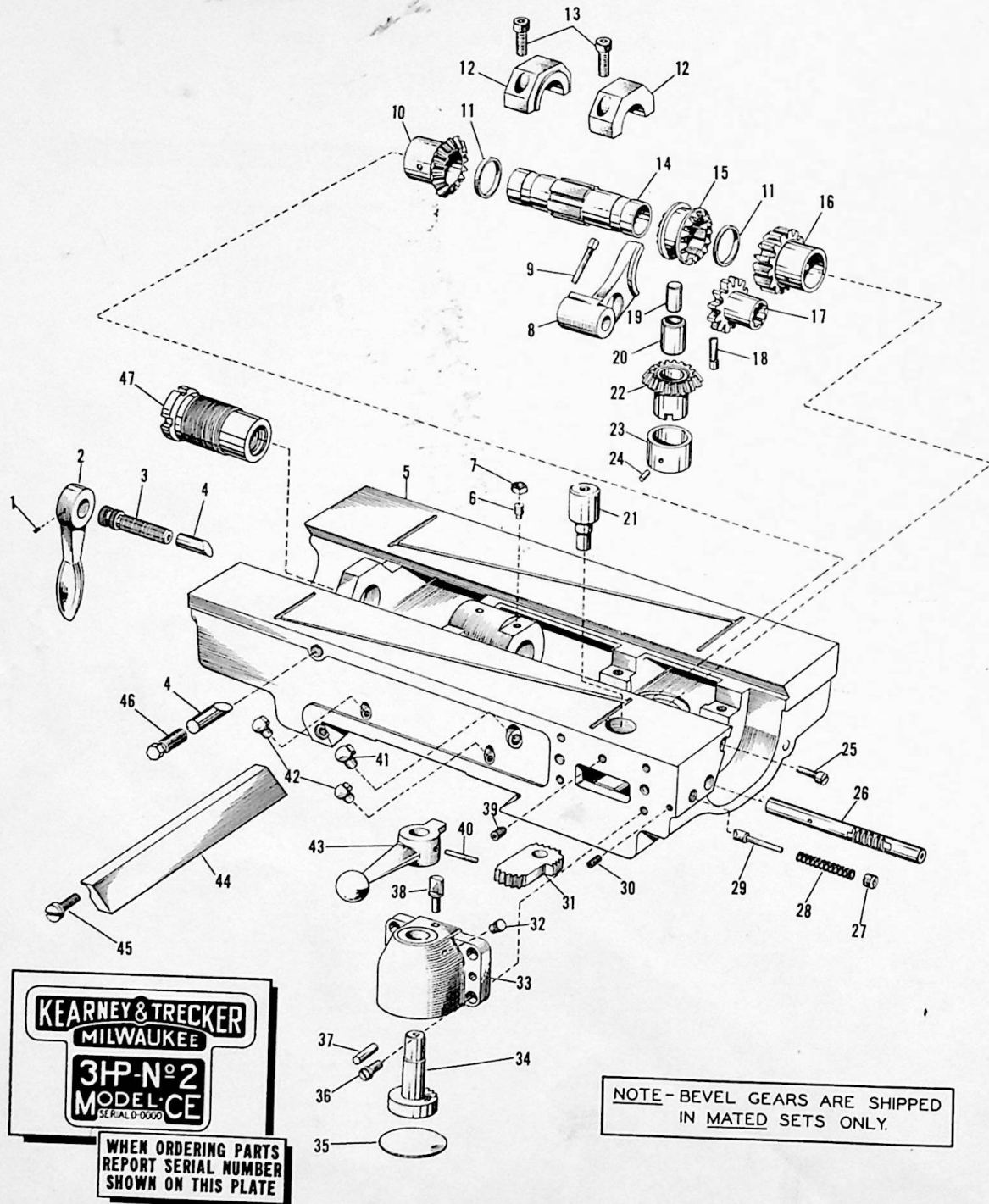
Fig. 12 — Plain Saddle assembly
