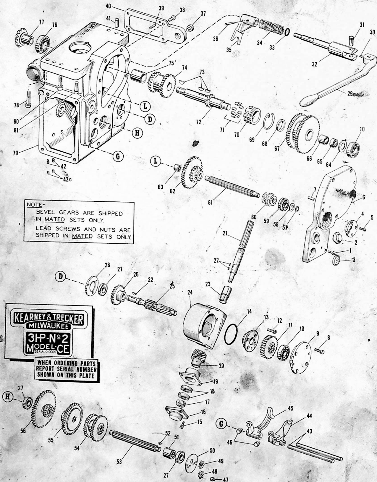
Fig. 11 — Feed gear box assembly — View B
