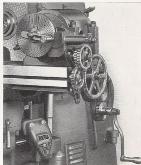
Figure 12 Enclosed Type Driving Mechanism for Dividing Heads.
