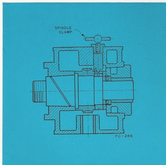
Figure 3 Longitudinal Section Showing Headstock Spindle Clamp
