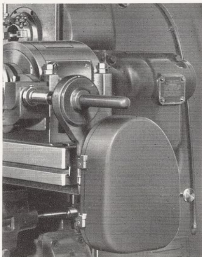
Figure 12 Enclosed Type Driving Mechanism for Dividing Heads.
