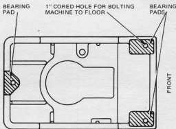
Figure M7B AREA ON UNDERSIDE OF BASE IN CONTACT WITH FLOOR
