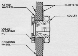
Figure M12 GRINDING WHEEL COLLET ASSEMBLY
