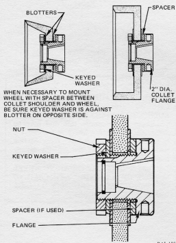
Figure M15B WHEEL ASSEMBLY AND SPACER LOCATION
