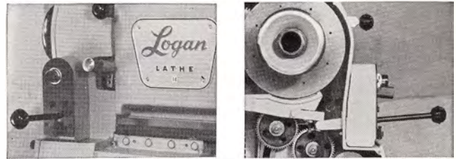
Downward movement of the brake lever stops lathe immediately. Push-button above brake lever re-starts lathe in same direction.
