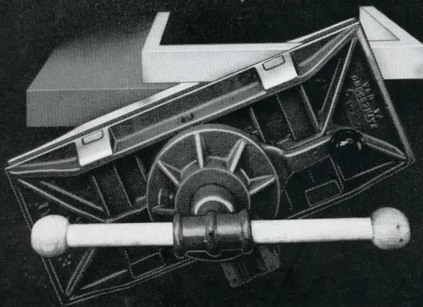
Jaws slightly rotated for holding boxes or drawers, etc., above or resting on bench top.
