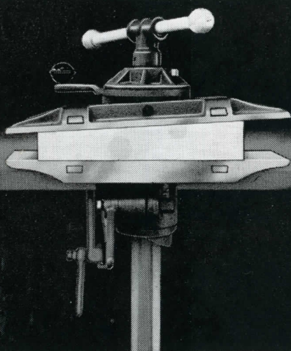
ROTO-VISE in upright position holding wedge shaped work at bench level.
