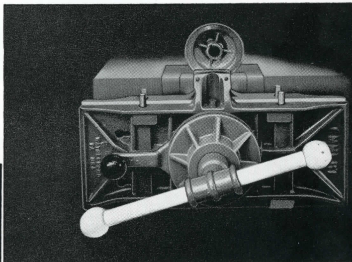
● Auxiliary, steel-faced jaws holding unusual and hard to grip work.
