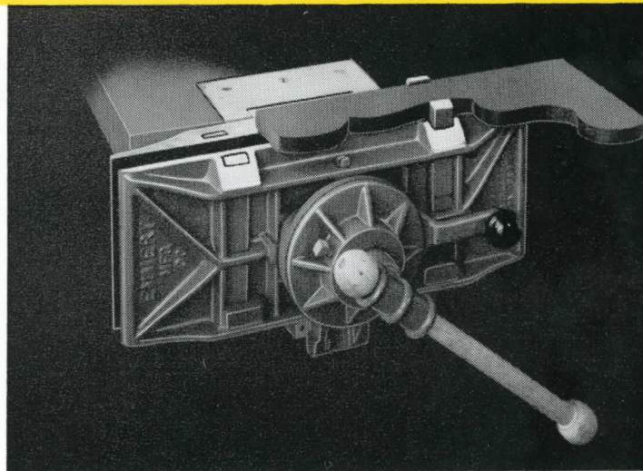
● Holding unusual shapes with the vise dogs. Either end of the jaw may be used, offering a flat or round holding surface.
