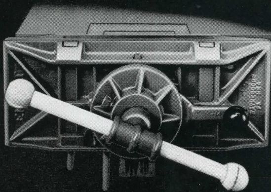
Normal position of ROTO-VISE, generally used to hold all simple rectangular shapes.
