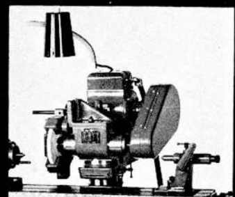
B955 UNIVERSAL GRINDING HEAD
