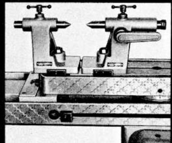
B922 TAILSTOCKS (MATCHED SET)
