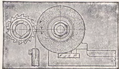
Grinding Clearance on a Cutter
