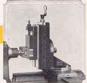
Fig. C—Vertical Vise Fixture
