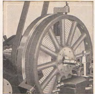
Boring a Wood Wheel. The wheel is mounted in a 3-jaw Universal Wheel Chuck. The hub can be fitted to the hole without removing the wheel from the lathe.
