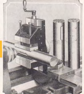
Milling a Keyway in Shaft
