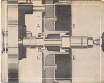
Timken Races and Universal Bearing Adapters A front wheel with Timken roller races, mounted on the mandrel fitted with universal bearing adapters, between centers in the lathe ready for testing or machining.
