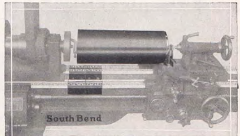
Double Bridge in Place Permits Using Lathe as a Straight Bed
