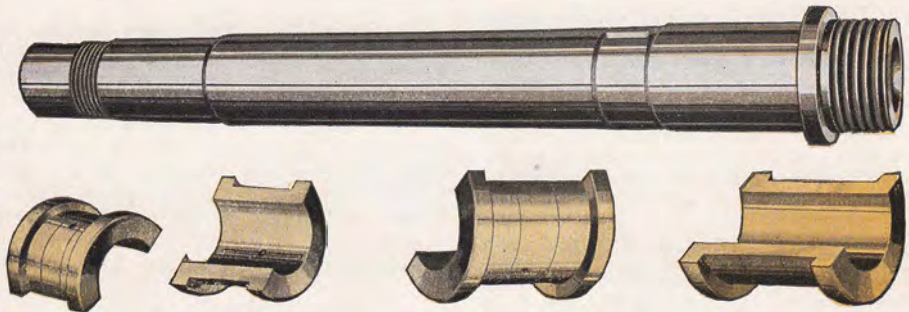
Scraping Bronze Bearings to Receive the Spindle
