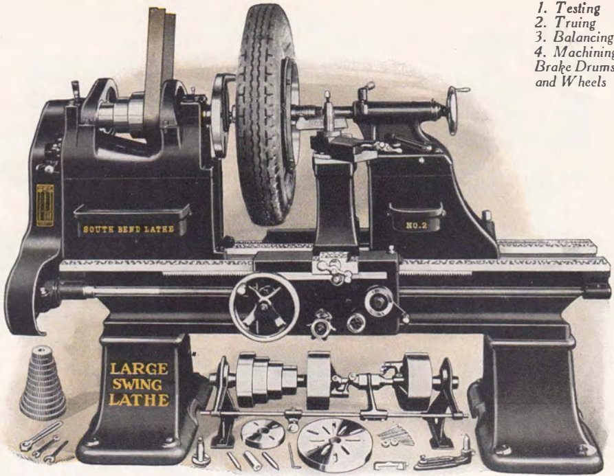
Countershaft and Equipment Included in Price of Lathe
