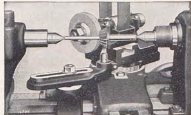
Grinding an Angular Cutter
