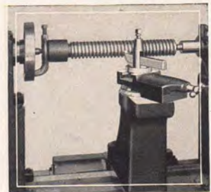
Cutting Screw Thread on a Jack Screw
