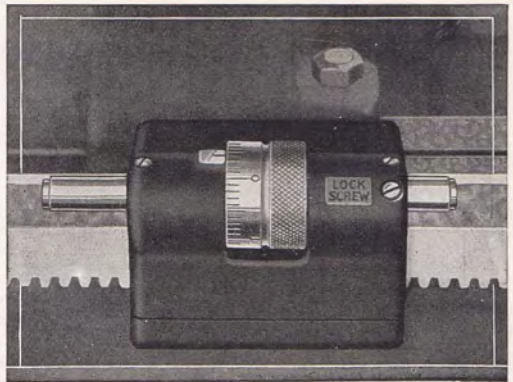
Micrometer Carriage Stop Fitted to Lathe Bed as a Permanent or Adjustable Stop
