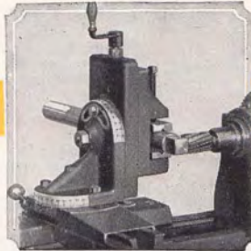
Fig. B—Squaring Steel Shaft
