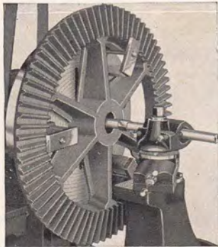
Boring Hole in a Large Bevel Gear Held in Wheel Chuck
