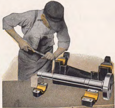
Scraping Bronze Bearings to Receive the Spindle
