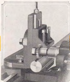
Milling a Standard Keyway
