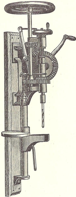
DRILL No. 3. Price, $22.00.
