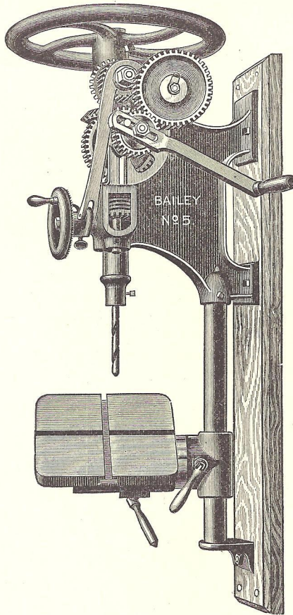
DRILL No. 5. Price, $36.00.
