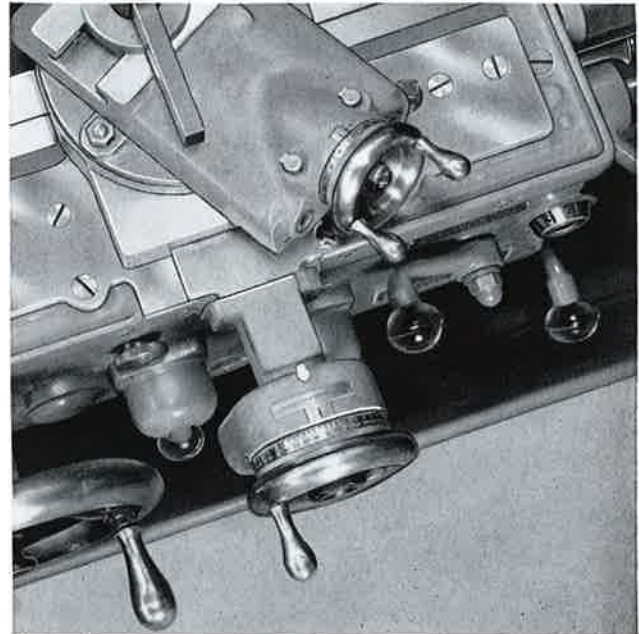
Large Direct-Reading Dials contribute to speed, accuracy and convenience in operation. The easy-to-read graduations give work diameter reductions in thousandths of an inch on the cross slide and on the compound rest.
