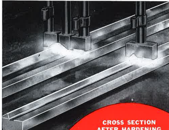
Left: Flame hardening process, showing all but the ways of a bed casting submerged in water.
