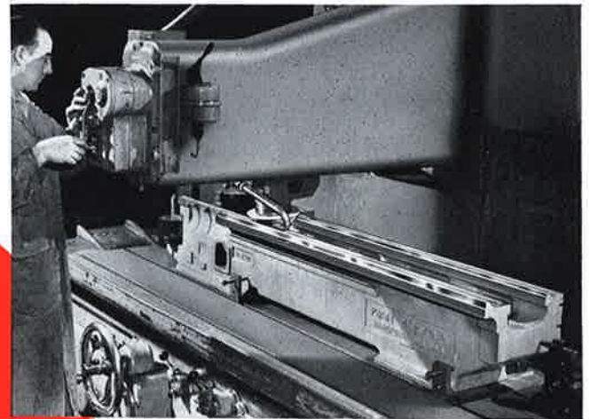
Finish grinding the front V-way of a Model "C" Lathe. All ways are accurately ground with the total end-to-end error not exceeding .0002".
