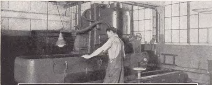
Powerful, accurate grinding machines insure absolute accuracy of all flat surfaces. All jointer tables are ground twice; once individually in accurate fixtures, then again after assembly with base, to assure precise alignment of finished machine.
