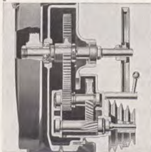
Gear drive is simple, foolproof and substantial and with self-sealed ball bearings is engineered for long life.
