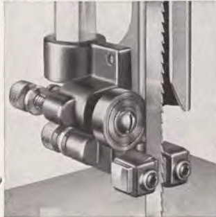
Micrometer adjustments of guides insure proper blade support for accurate work yet allow blade to run free.
