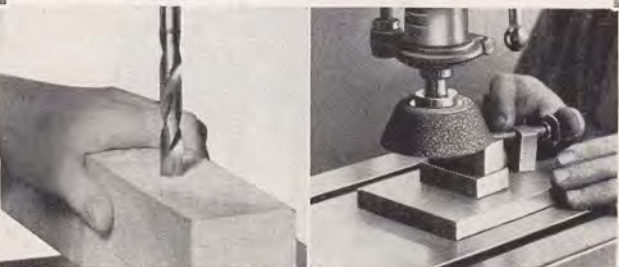
Boring in wood with spur bits is practical because of the standard high speeds.
