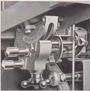
Showing massive and accurate construction of the lower guide control and front table trunnion (Patent Pending).
