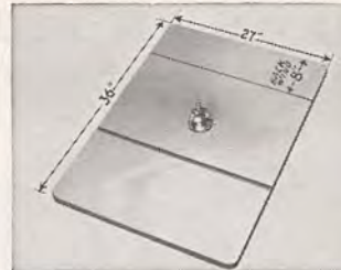
Large table 27" x 28" may be increased to 27" x 36" by addition of back wing. Bolting two shapers together produces a 2-spindle machine with a table 27" x 4'-8".
