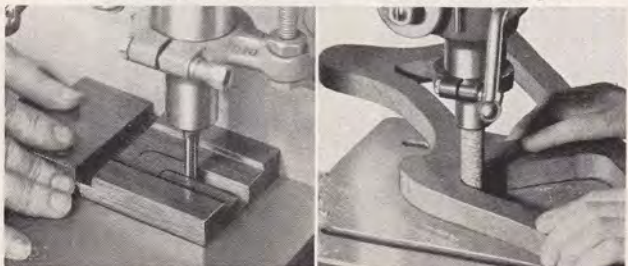
The routing of all kinds of grooves is made simple, using standard router bits.
