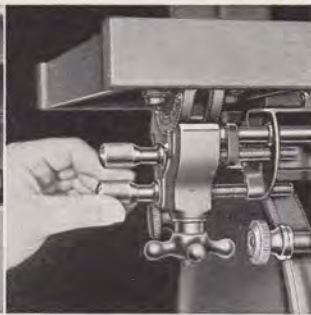
Lower guide control adjustment brought to front of table so that operator's hands need not come near blade.
