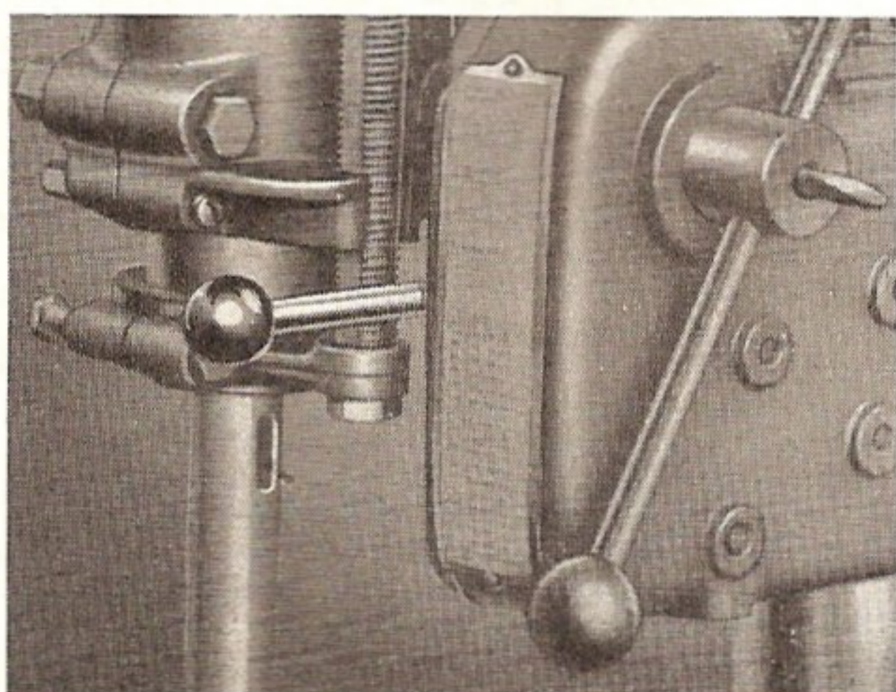
Operating Power Feed Handle is conveniently located.
