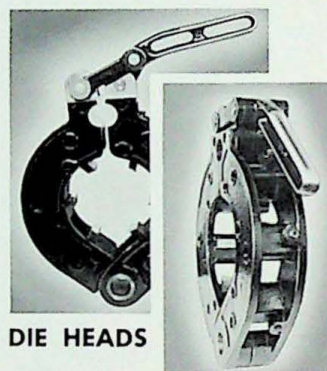
THREADING
