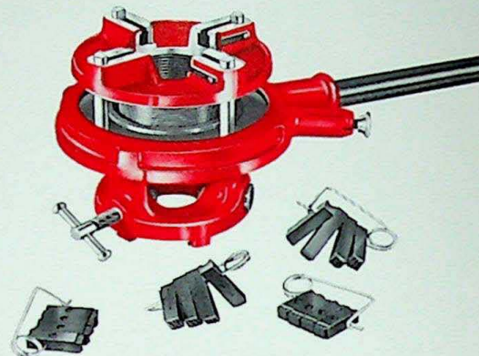
COMPLETE TOOL WITH R.H. DIES
