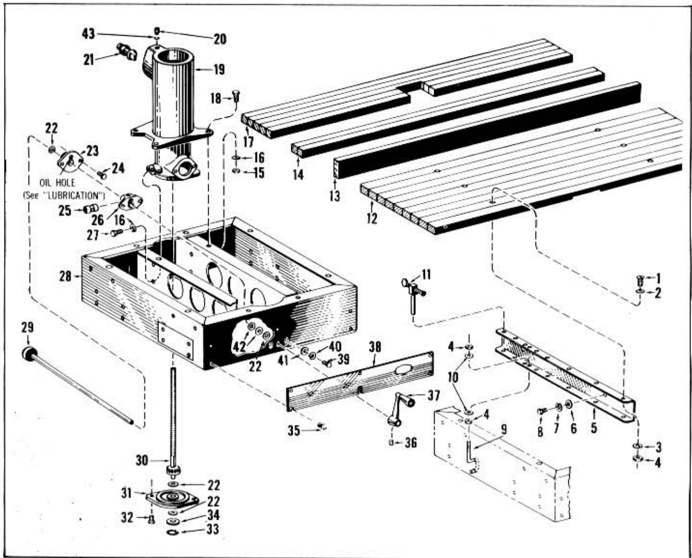
FIGURE 2 PARTS LIST
